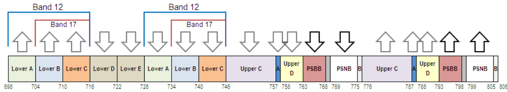
Figure 1: Lower 700 MHz Band with Bands 12 and 17
