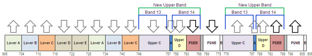
Figure 2: Upper 700 MHz Band and Bands 13, 14, and New Upper Band
