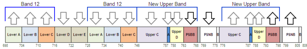
Figure 3: Upper and Lower 700 MHz Bands
